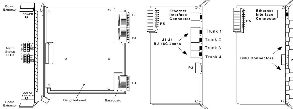
Faceplate (front view)
